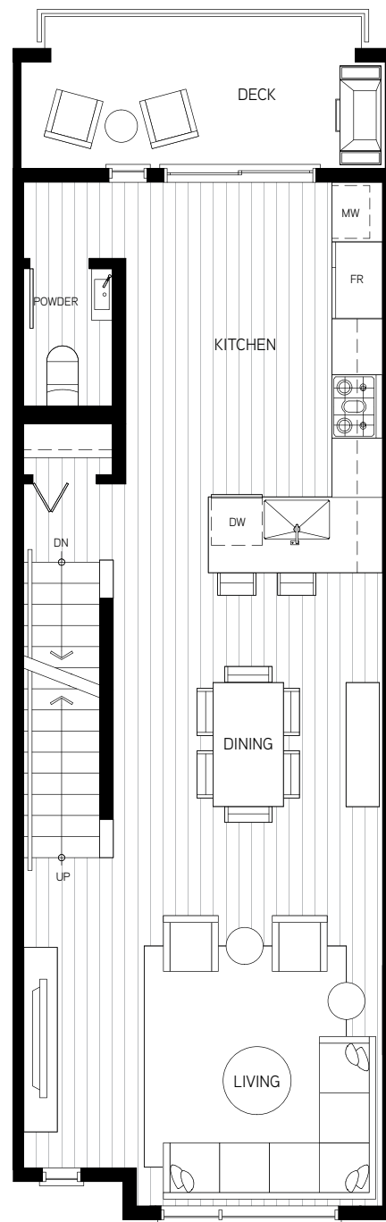
MAIN FLOOR
